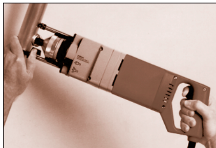
FIGURE 33: Tee-Pulling Tool
