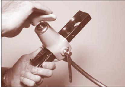
FIGURE 31: Lowering the Flaring Cone into the Tube End
